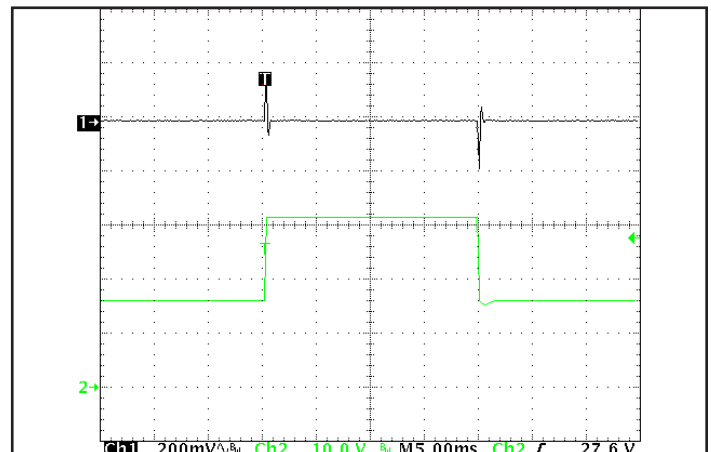
Figure 6: Output voltage response to step-change in input voltage (nominal to maximum; 250 V/ms). Load cap: 1 \mu F ceramic, 15 \mu F tantalum, and 100 \mu F electrolytic cap. Ch 1: Vout (200 mV/div), Ch 2: Vin (10 V/div). Timebase: 5.00ms/div.
