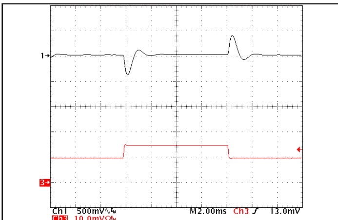
Figure 5: Output voltage response to step-change in load current (50-75-50% of I_{out(max)} ; dI/dt = 0.1 A/\mu s ). Load cap: 1 \mu F ceramic, 15 \mu F tantalum, and 100 \mu F electrolytic cap. Ch 1: V_{out} (500 mV/div), Ch 3: I_{out} (0.5 A/div). Timebase: 2.00ms/div.
