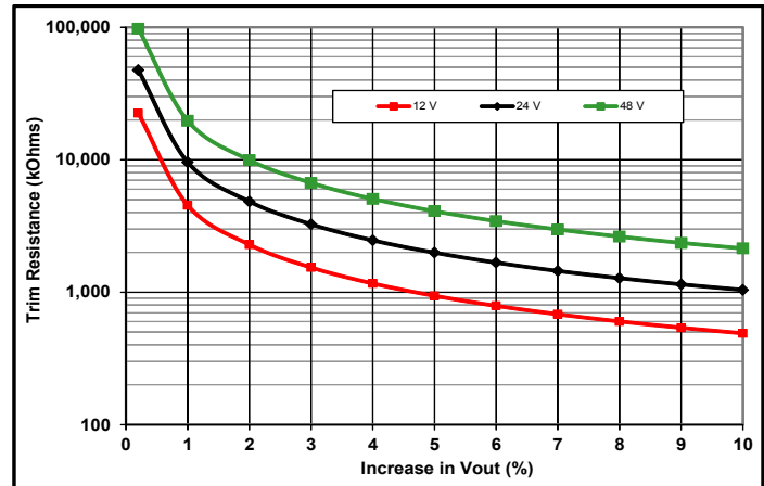
Common Figure 4: Trim graph for trim-up 12 to 48V outputs.
