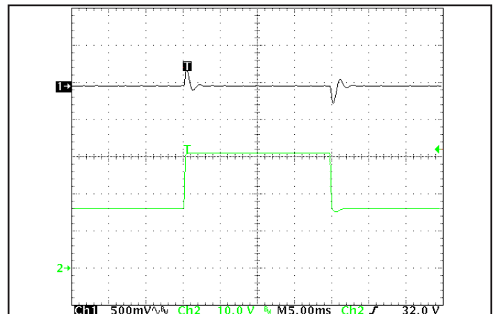
Figure 6: Output voltage response to step-change in input voltage (nominal to maximum; 250 V/ms). Load cap: 1 \mu F ceramic, 15 \mu F tantalum, and 100 \mu F electrolytic cap. Ch 1: V_{out} (500 mV/div), Ch 2: V_{in} (10 V/div). Timebase: 5.00ms/div.
