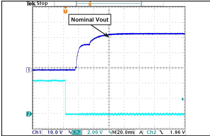
Common Figure 1: Typical startup waveform. Input voltage pre-applied, Ch 1: Nominal Vout, Ch 2: ON/OFF Pin (2 V/div). Timescale: 20.0ms/div.
