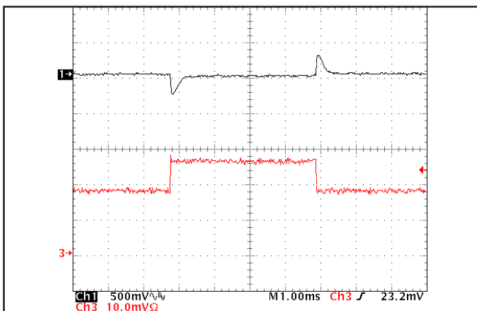
Figure 5: Output voltage response to step-change in load current (50-75-50% of I out (max)); dI/dt = 0.1 A/μs. Load cap: 1 μF ceramic, 15 μF tantalum, and 100 μF electrolytic cap. Ch 1: V out (500 mV/div), Ch 3: I out (1 A/div). Timebase: 1.00ms/div.
