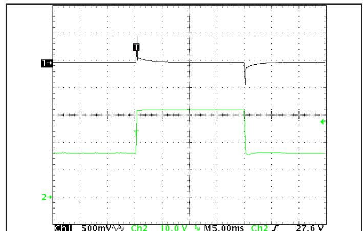
Figure 6: Output voltage response to step-change in input voltage (nominal to maximum; 250 V/ms). Load cap: 1 μF ceramic, 15 μF tantalum, and 100 μF electrolytic cap. Ch 1: V out (500 mV/div), Ch 2: V in (10 V/div). Timebase: 5.00ms/div.
