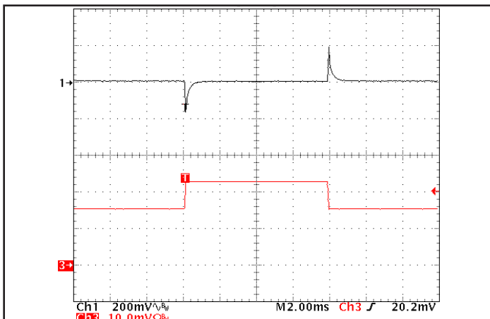
Figure 5: Output voltage response to step-change in load current (50-75-50% of Iout(max)); dI/dt = 0.1 A/\mu s . Load cap: 1 \mu F ceramic, 15 \mu F tantalum, and 100 \mu F electrolytic cap. Ch 1: Vout (200 mV/div), Ch 3: Iout (5 A/div). Timebase: 2.00ms/div.
