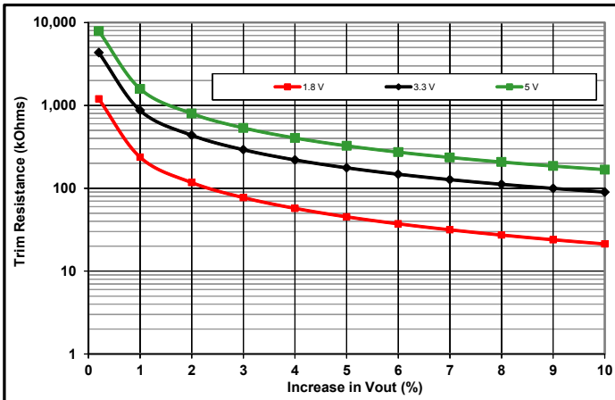
Common Figure 3: Trim graph for trim-up 1.8 to 5V outputs.
