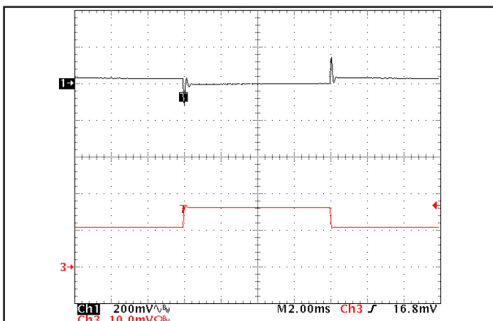
Figure 5: Output voltage response to step-change in load current (50-75-50% of I out (max); dI/dt = 0.1 A/μs). Load cap: 1 μF ceramic, 15 μF tantalum, and 100 μF electrolytic cap. Ch 1: V out (200 mV/div), Ch 3: I out (10 A/div). Timebase: 2.00ms/div.
